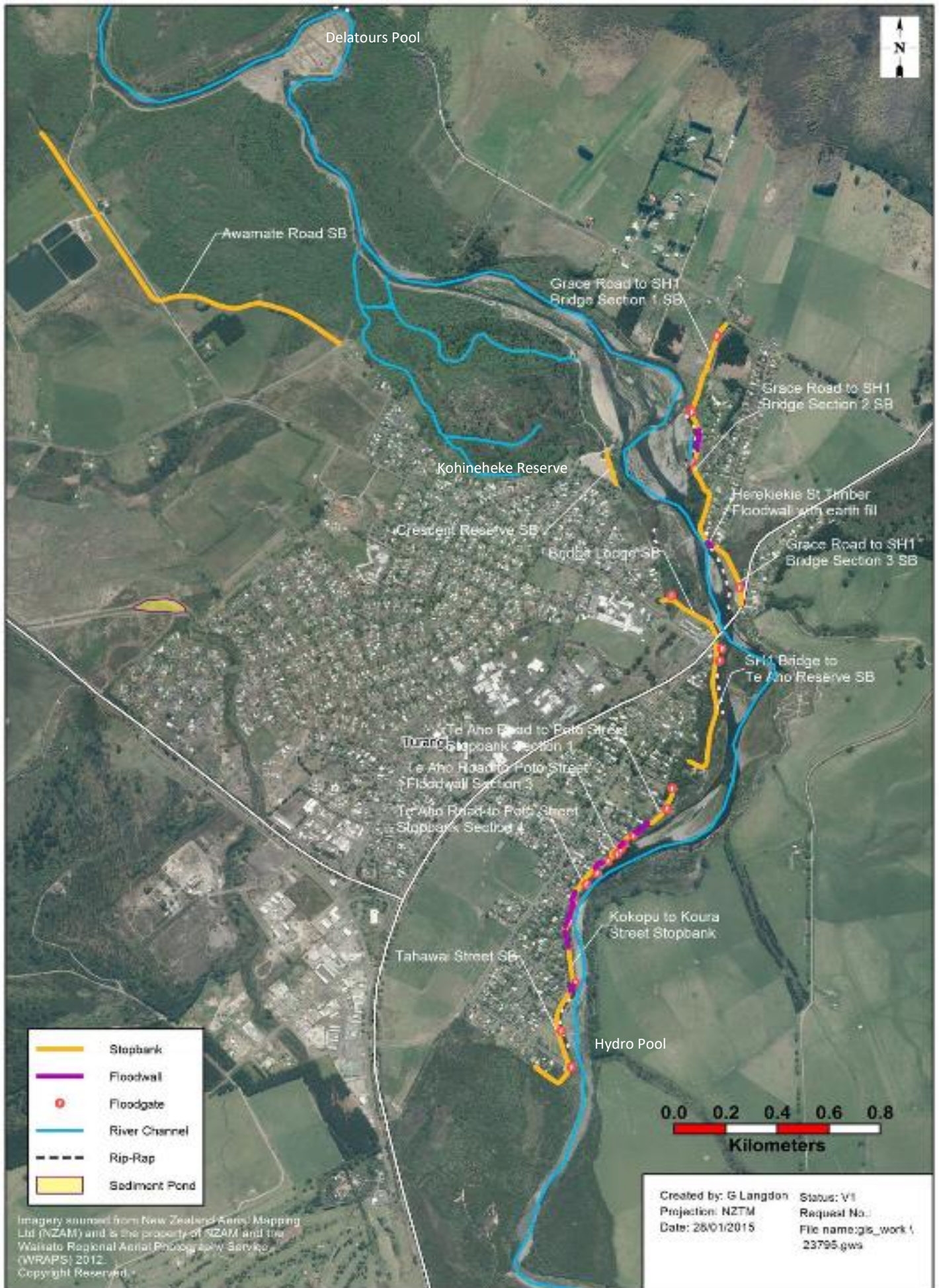
Figure 1: Tongariro River Flood Control Scheme
