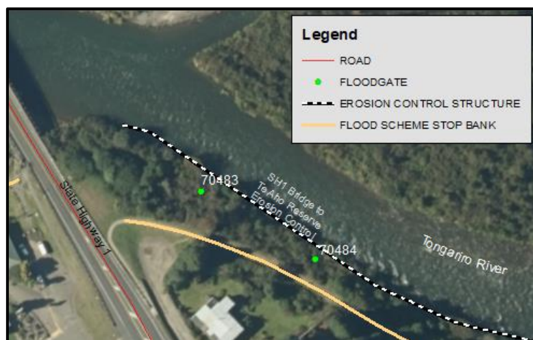
Figure 2: SH1 Bridge to Te Aho Reserve rock protection and Floodgate Flap Valves location.
